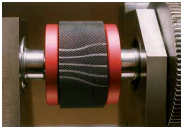
OGEE LINES UNDER NO LOAD.
