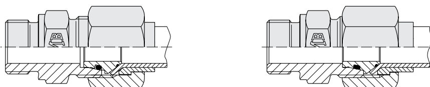
Before tightening the nut
