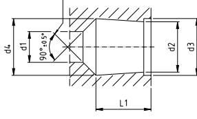
Bore (RVS 6-L/S / 8-S only) Bore (must align exactly)
